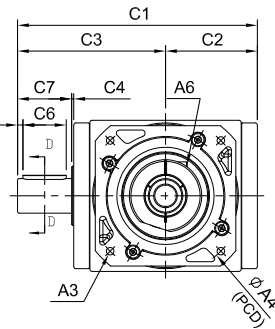
R 軸 Shaft Direction
