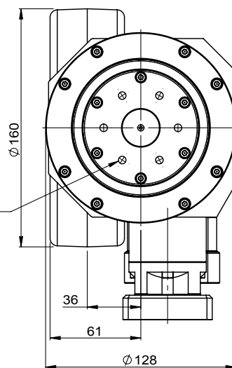
PCD50 6-M6X1.0 Deep12
